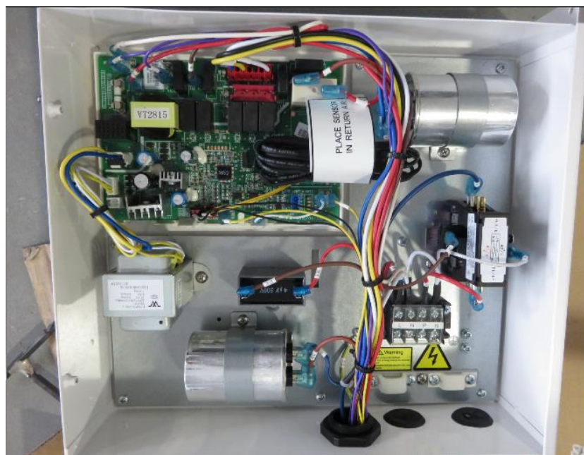
Main power box
