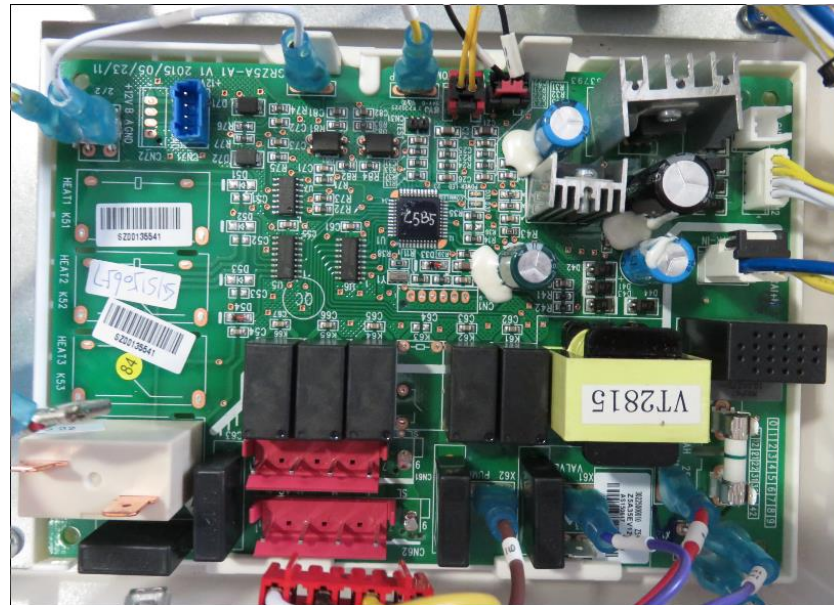
Main board
