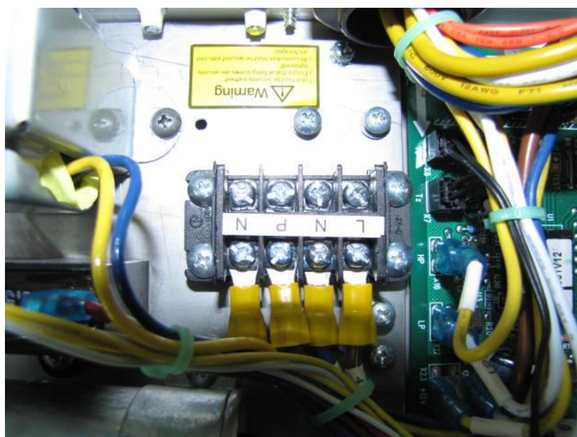
Terminal board view
