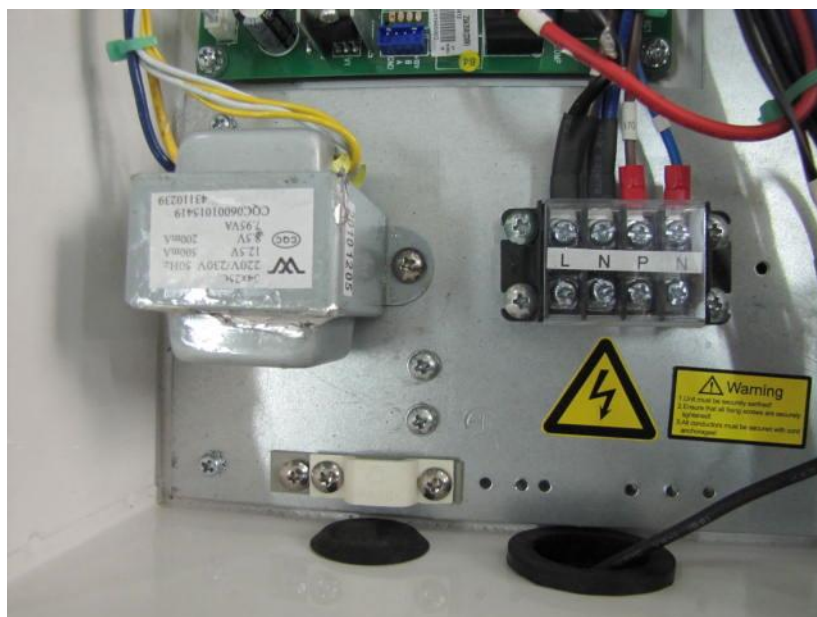
Cord anchorage, earthing terminal and terminal board view
