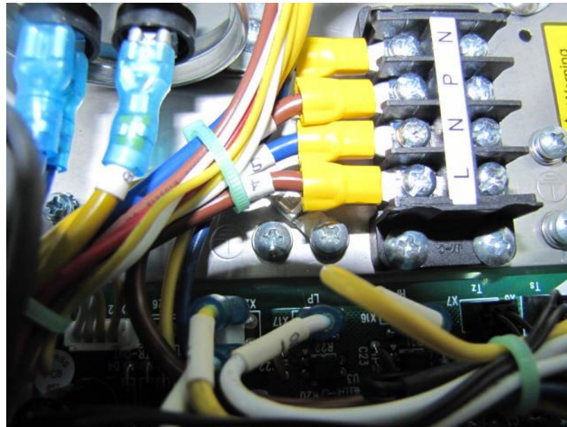
Earthing terminal view
